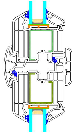
AA -1-2 DETAYI
