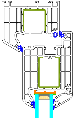
AA -2 DETAYI
