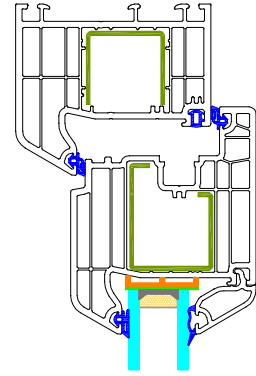
AA -1 DETAYI
