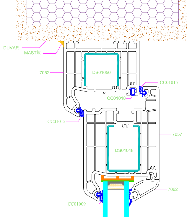
AA - DETAYI
