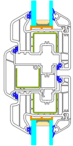
AA - DETAYI
