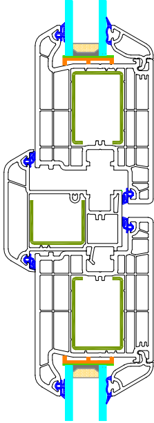
AA - DETAYI
