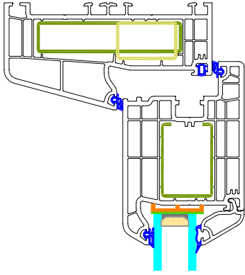
AA - DETAYI
