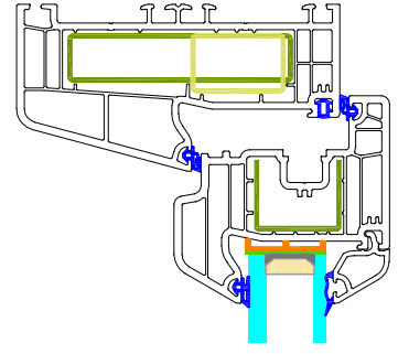
AA - DETAYI
