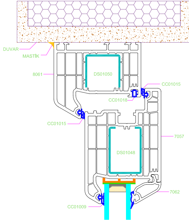
AA - DETAYI
